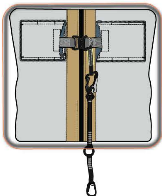
Belt connection front view
